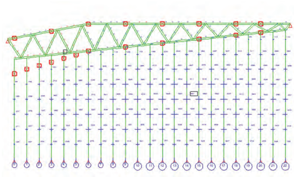
Figure 2-2 Grand Egyptian Museum, Cairo (Egypt). Structural analysis of one of the six cable facades. (© Werner Sobek AG)
